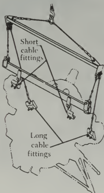
FIGURE 8-24. Special sling used for hoisting helicopter QECA.
